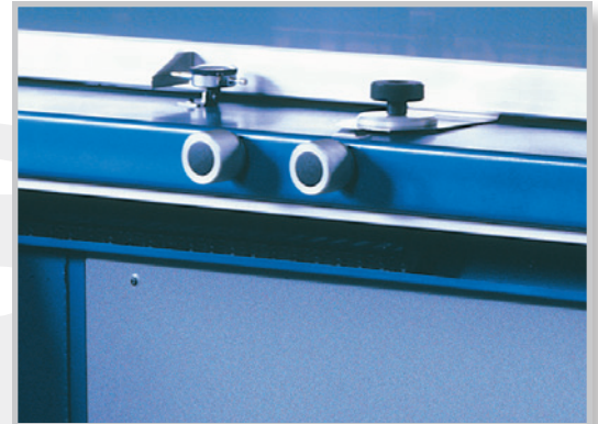
Vacuum bed dial indicators measure movement in .0025 cm (.001") increments
